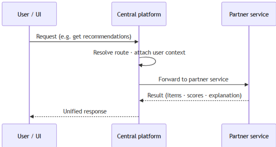
Figure 5. A service request, end to end
