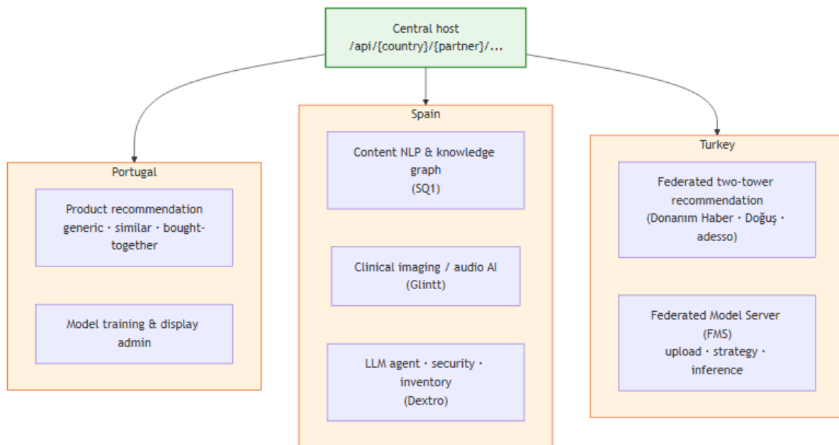
Figure 4. Unified service catalogue by country and function
