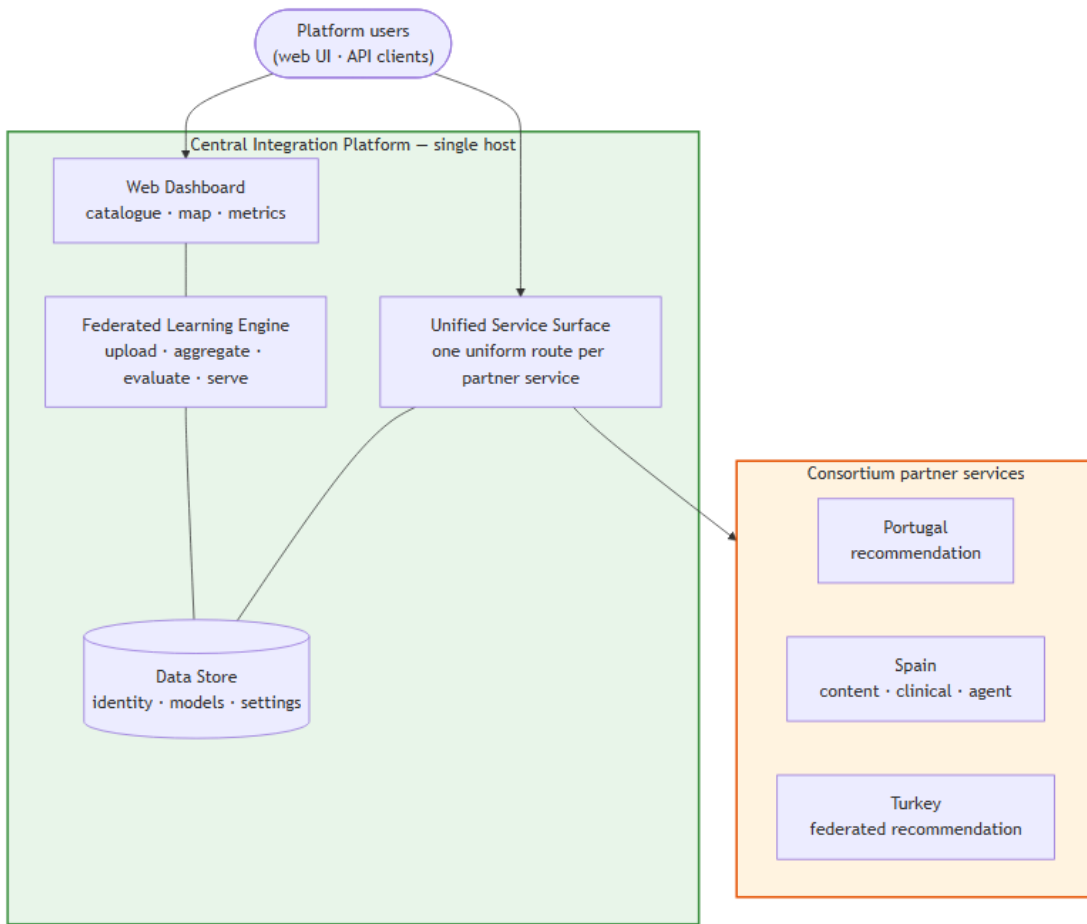
Figure 1. High-level software composition
