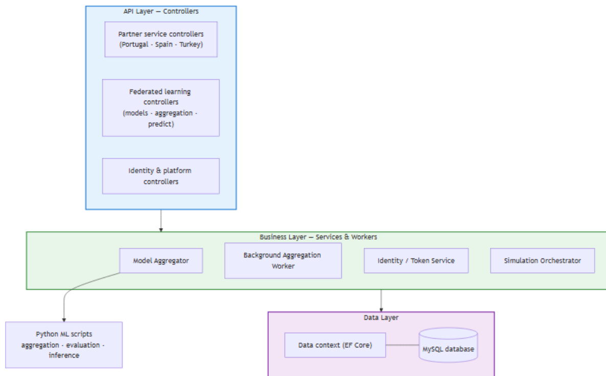
Figure 2. Backend component and layer map
