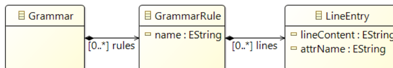
Figure 6: The class design for grammar rules.
