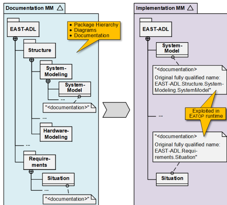
Figure 2: General Approach for Transforming an EAST-ADL Documentation MM to an EATOP Implementation MM
