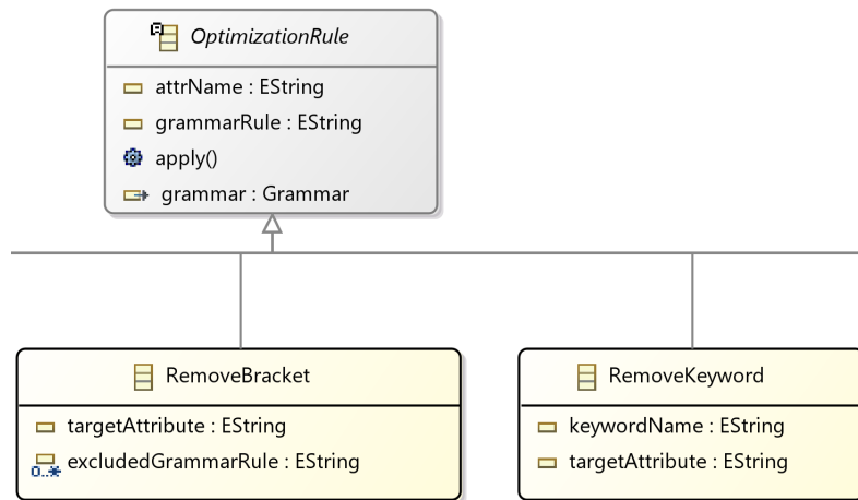
Figure 7: Excerpt of the class diagram for optimization rules.
