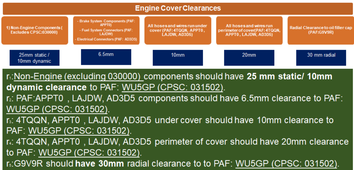
Figure 4. Example Clearance Specification.
