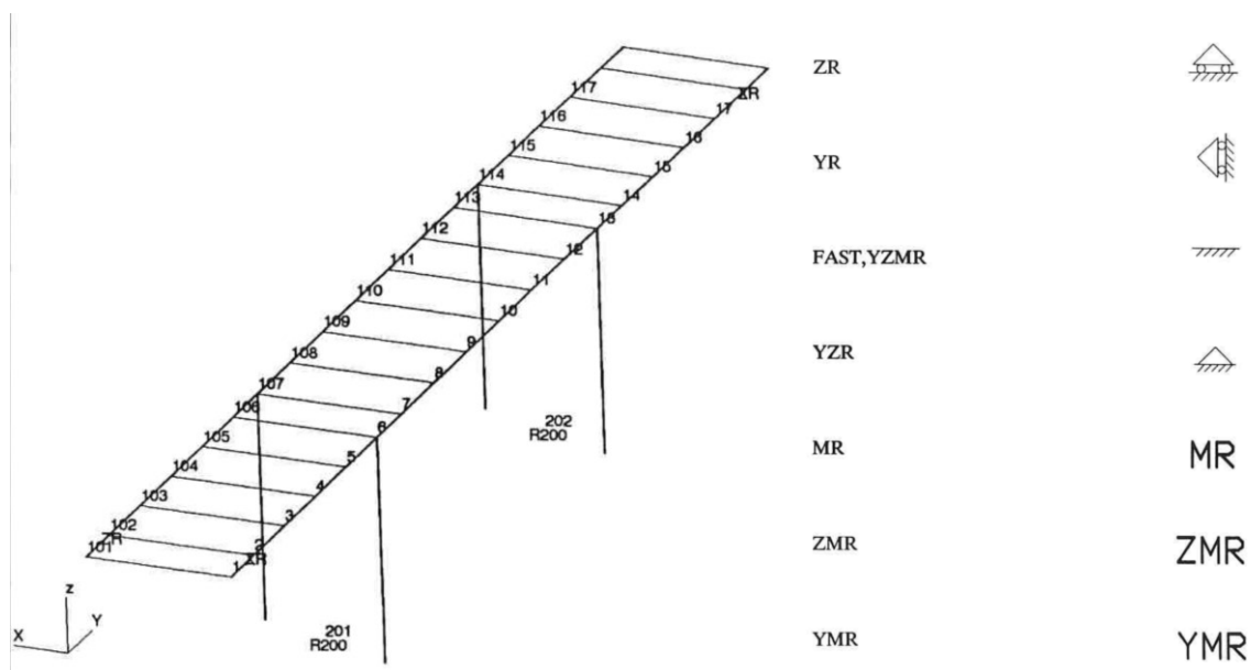
Figure 5. Example graphical view for a DSML instance.
