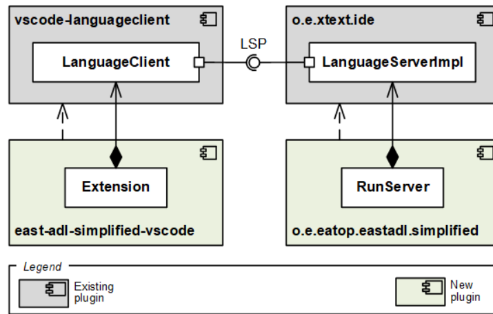
Figure 13: Architecture for bringing the EATXT editor to VS Code and Eclipse Theia via LSP
