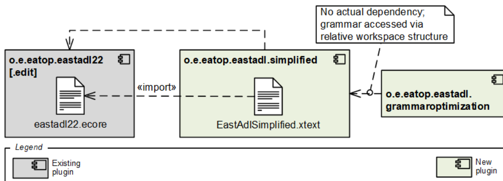
Figure 14: Architecture for the post-processing of the EATXT grammar
