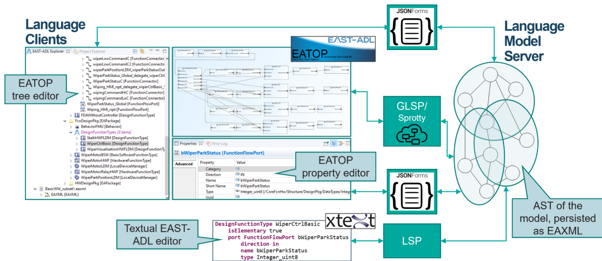
Figure 12: Vision of blended EAST-ADL modeling based on different LSP frameworks
