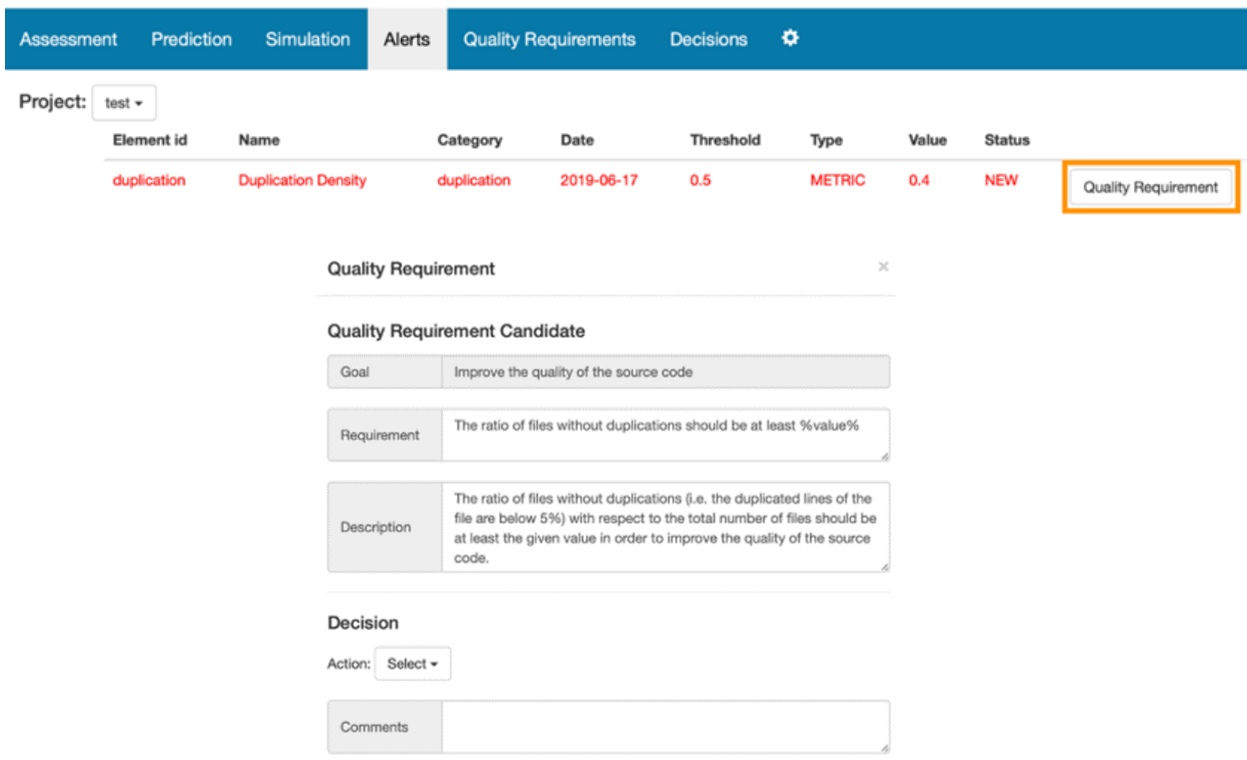
Figure 40. QaSD quality alert and QR suggestion
