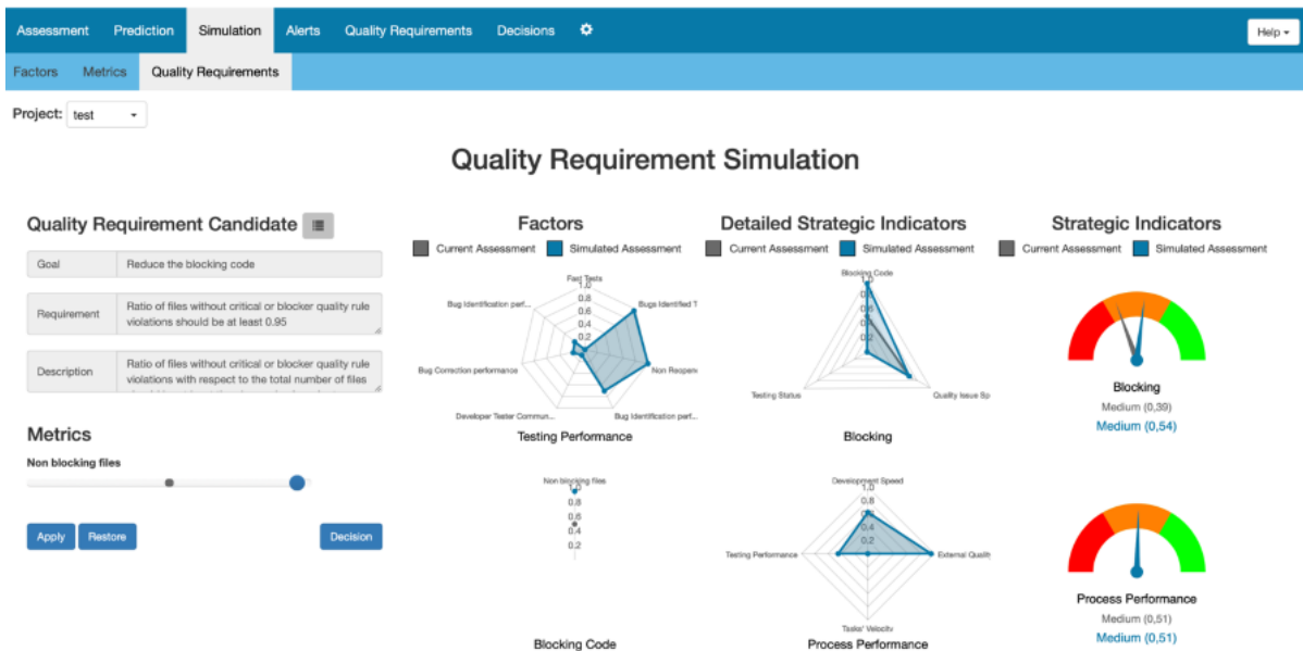
Figure 41. Q-Rapids QR simulation
