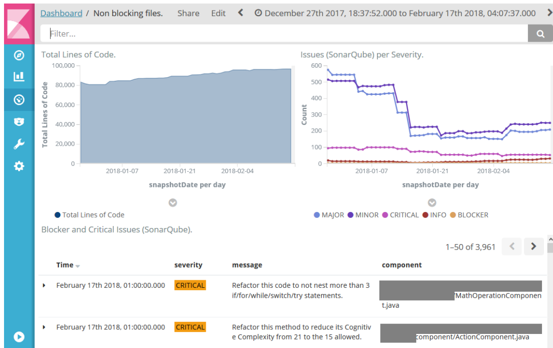
Figure 37. Q-Rapids Raw Data dashboard
