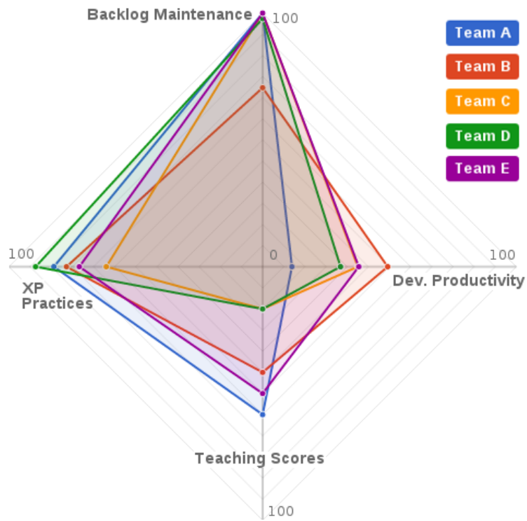
Figure 7: Radar chart provided by ScrumLint (Matthies et al., 2016).
