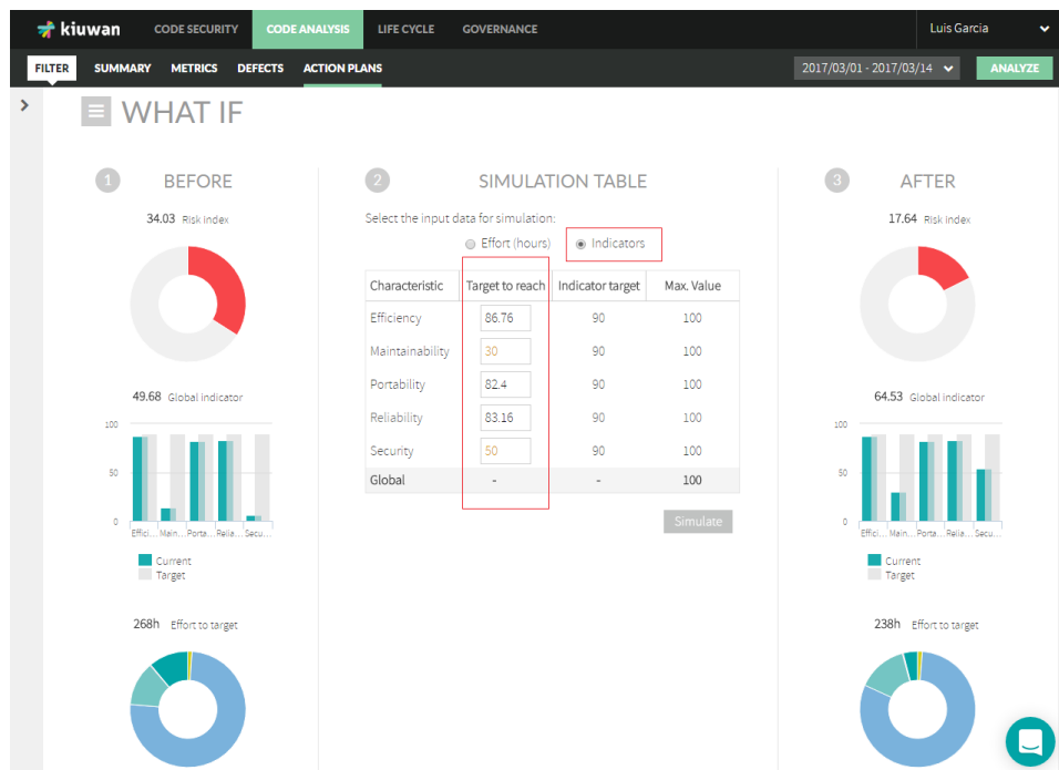
Figure 14. Kiuwan simulation feature
