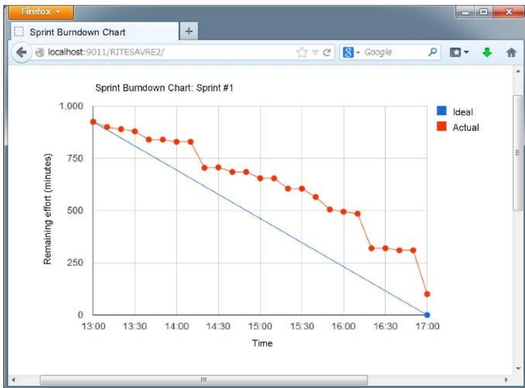
Figure 4: Sprint burndown chart (Igaki et al., 2014)
