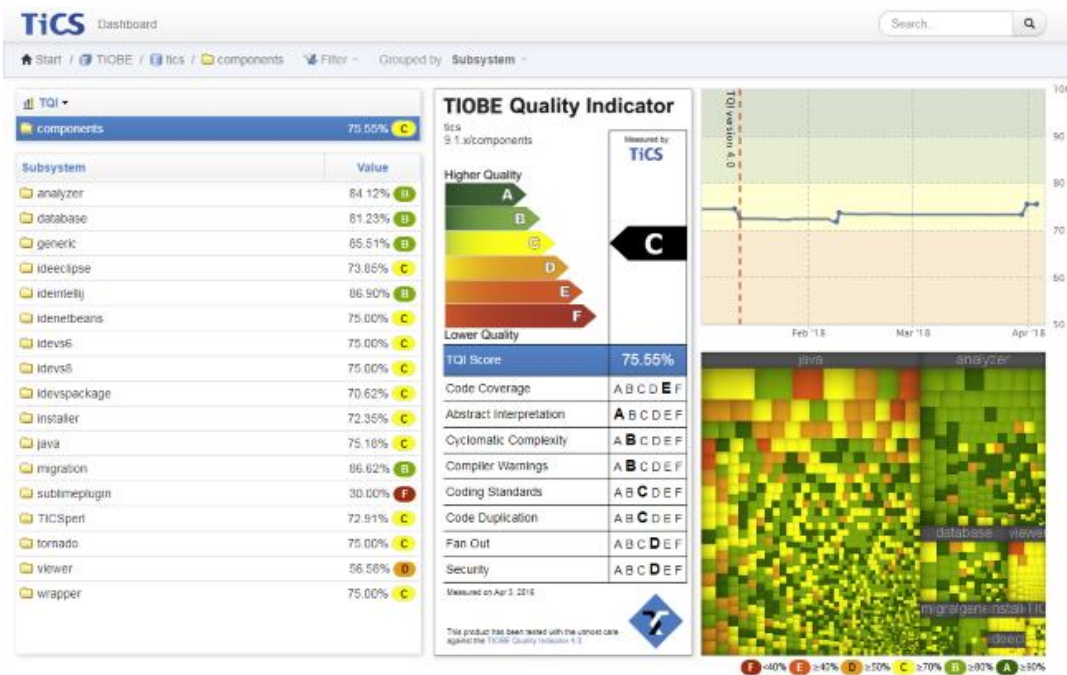
Figure 28: TiCS Framework Dashboard
