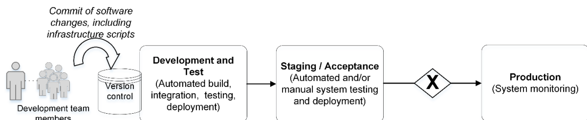
Figure 8: Continuous deployment pipeline
