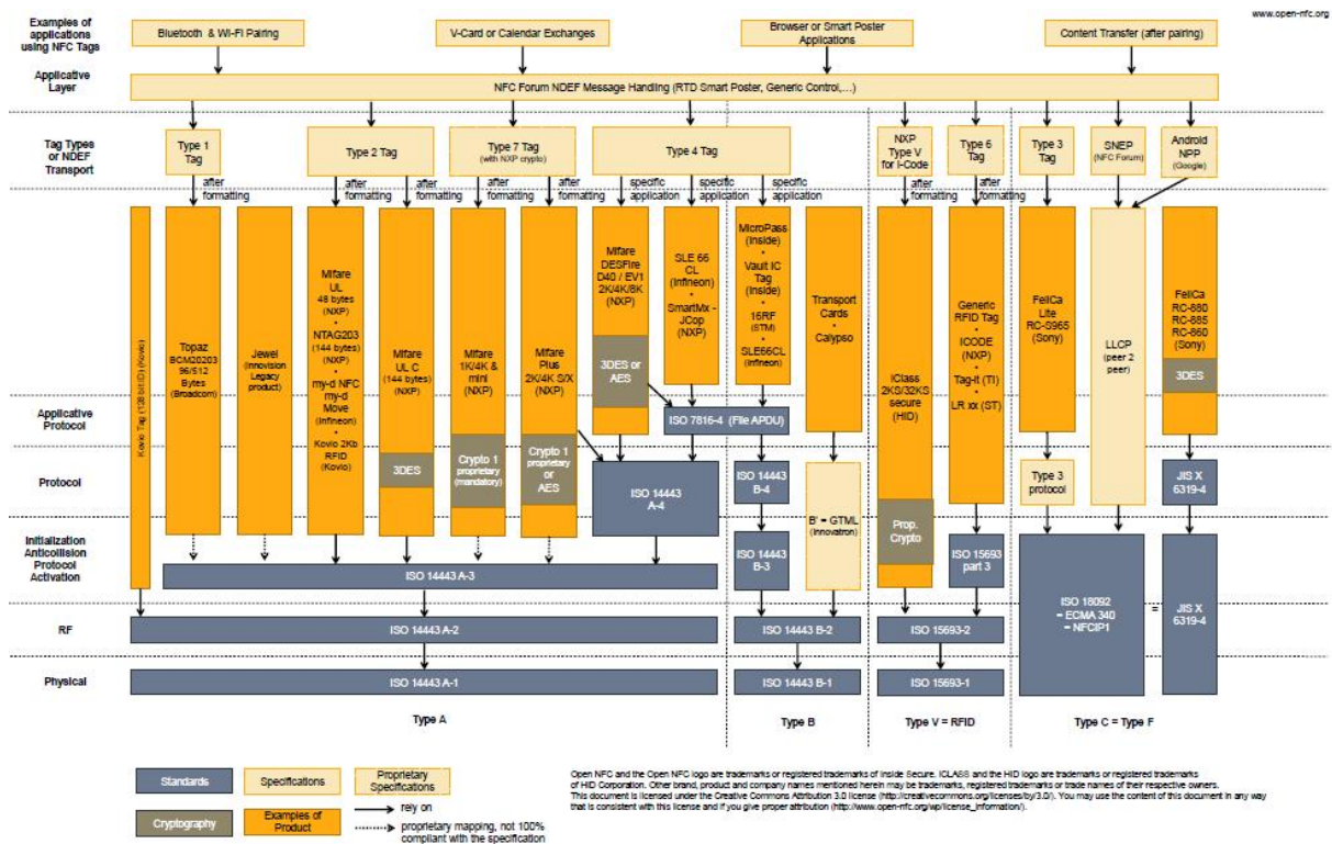
Figure 39: NFC architecture
