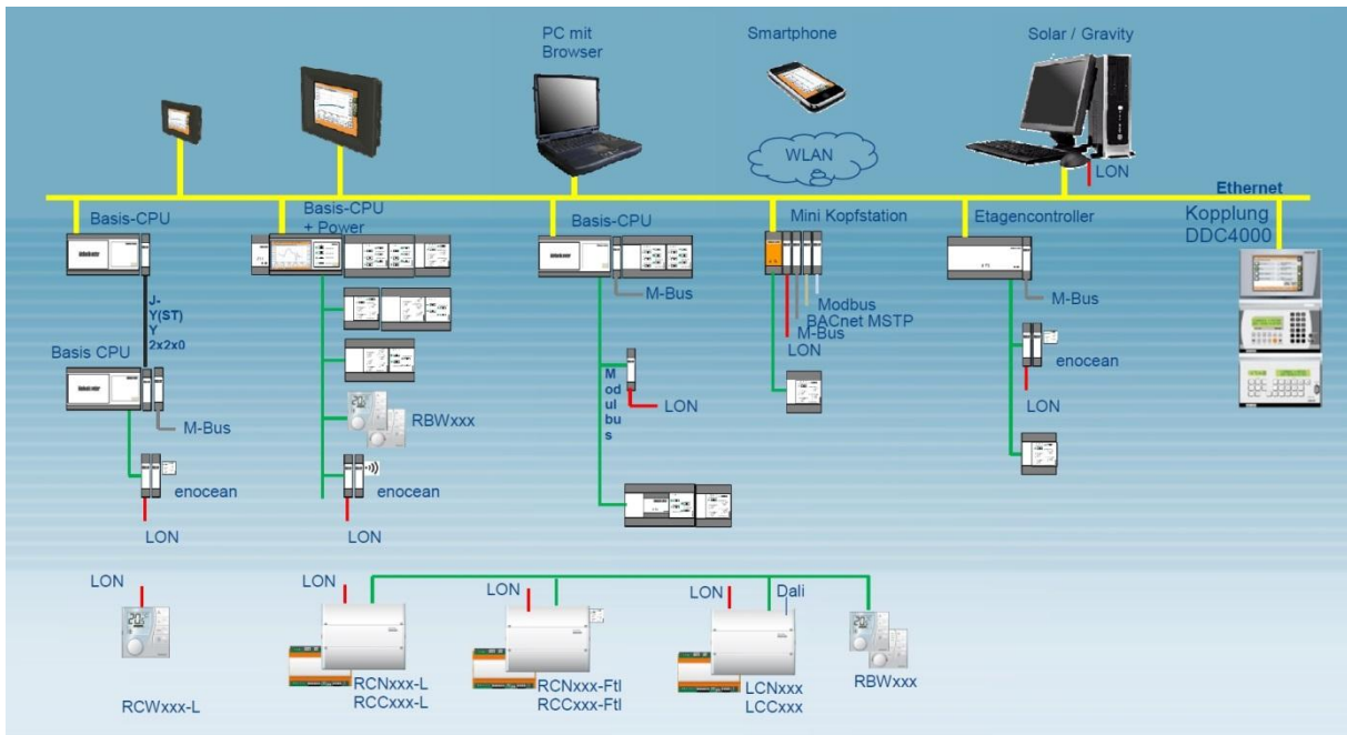
Figure 4: System topology within the Kieback&Peter company (new automation system, Source: Kieback&Peter GmbH & Co. KG)
