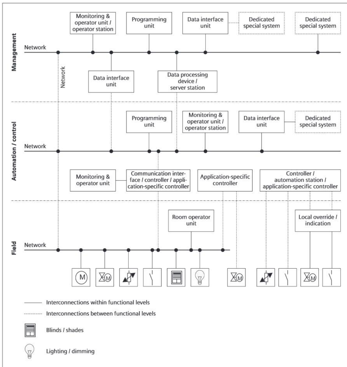
Figure 3: Possible interconnections in three-level functional hierarchy
