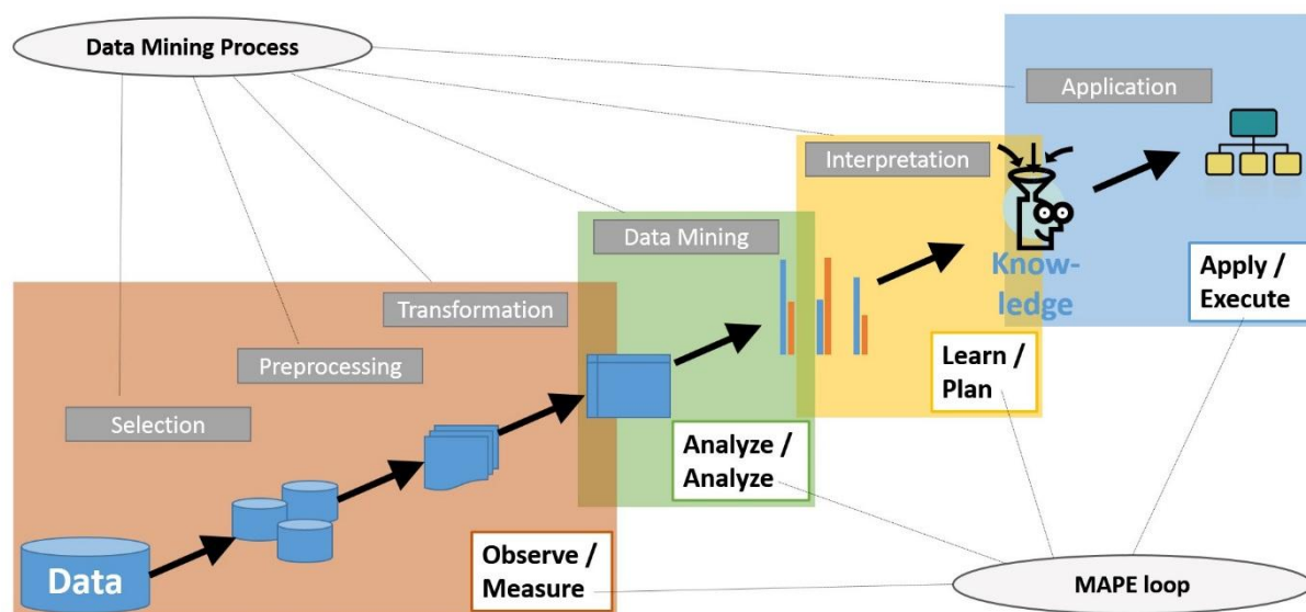
Figure 7: Data Mining Process adapted from [62] compared with the MAPE loop.
