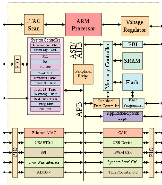
Figure 44: Block diagram of SoC
