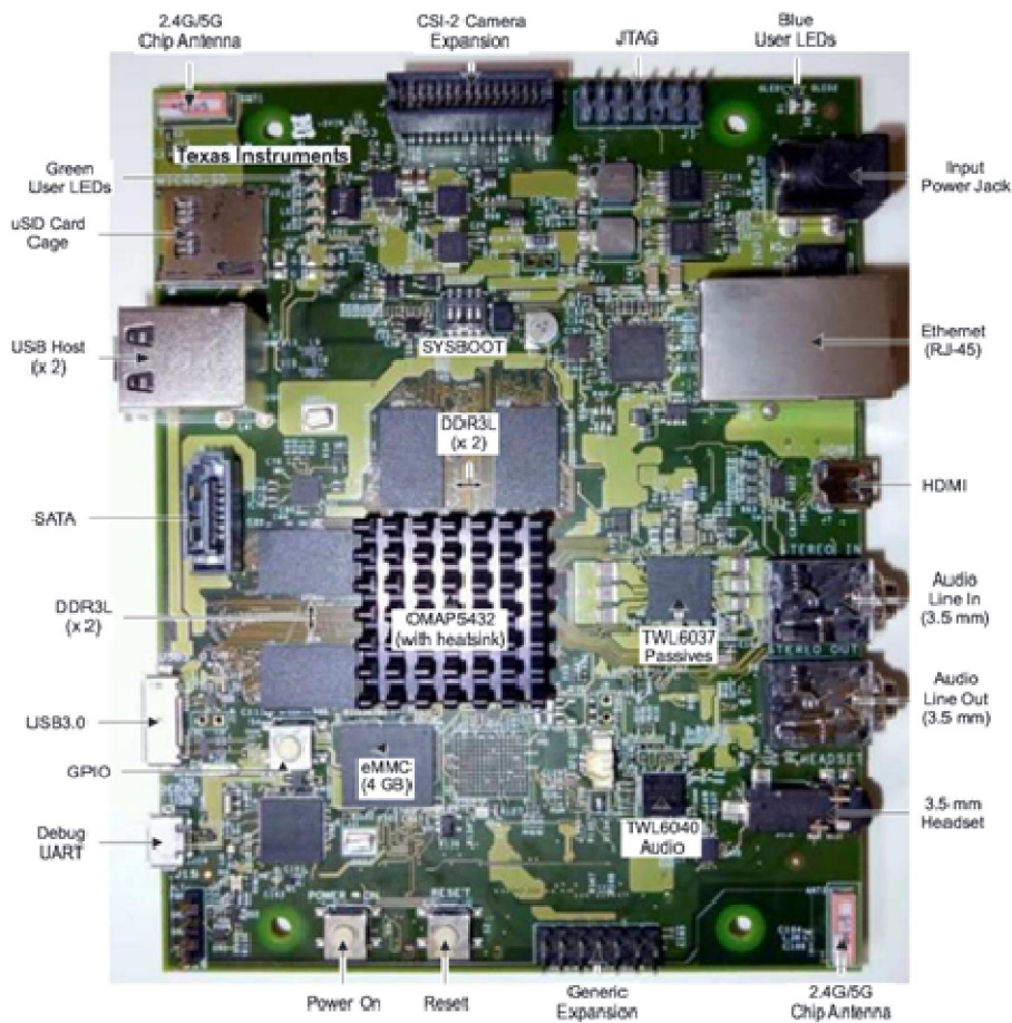
Figure 54: Singleboard computer OMAP5432 EVM
