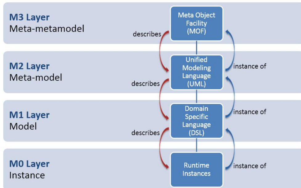
Figure 38: Example of the four-layered MOF Metamodel architecture
