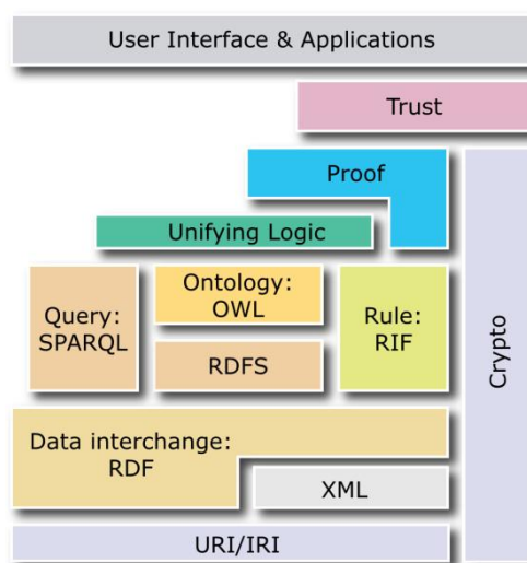
Figure 30: The Semantic Web Stack
