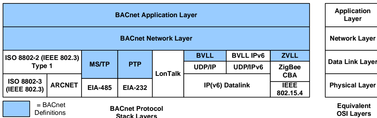
Figure 16: Collapsed BACnet Architecture.
