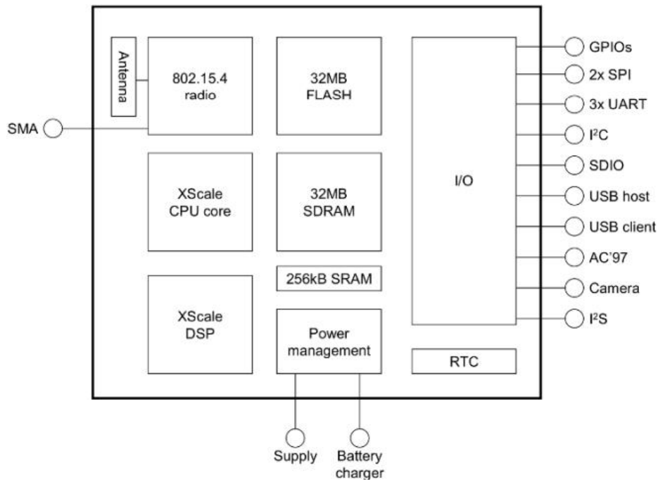
Figure 43: Block diagram of embedded computer Imote2
