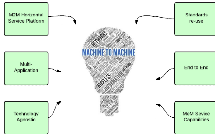
Figure 42: M2M
