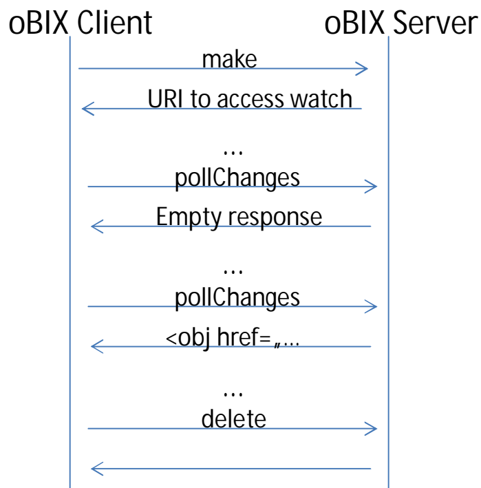
Figure 24: Watch lifecycle
