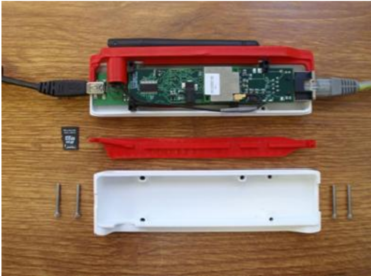
Figure 46: Uncovered firewall prototype microcomputer-based on Gumstix Verdex developed at Masaryk University
