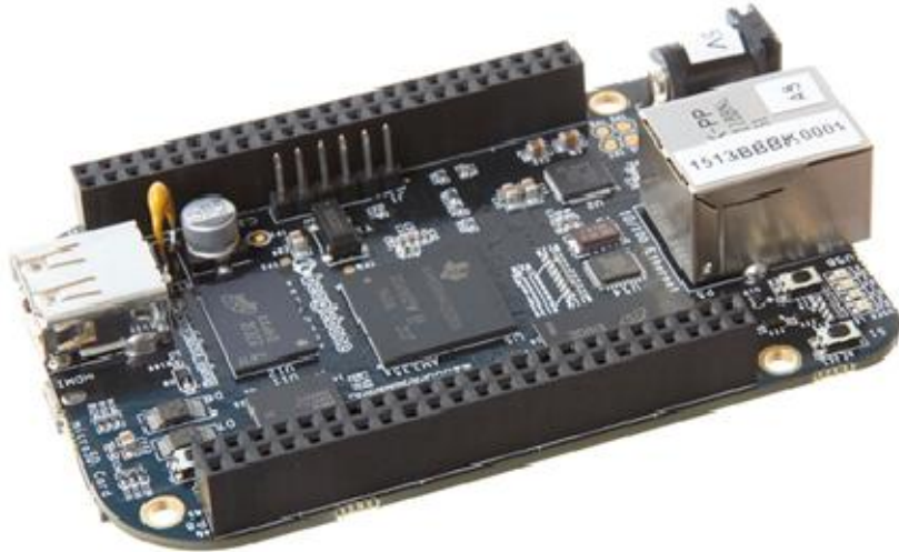
Figure 50: Single-board BeagleBone Black computer
