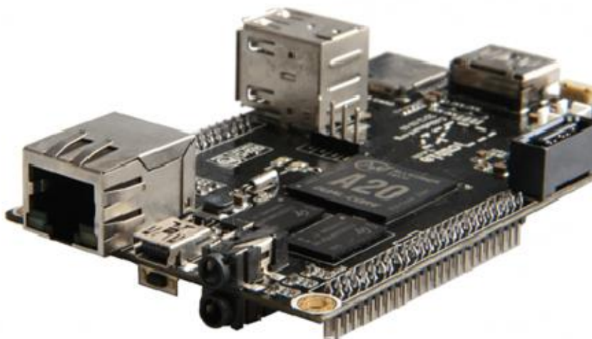
Figure 51: Single-board computer Cubieboard2
