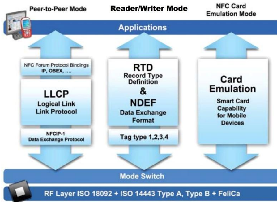
Figure 40: NFC Standard
