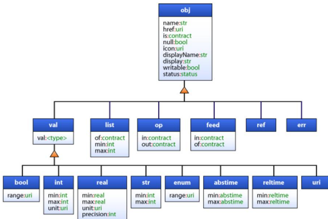
Figure 20: Object Model
