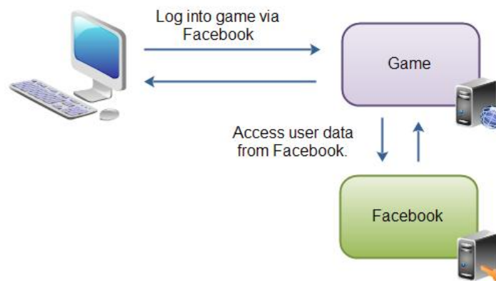
Figure 10: Example of how OAuth 2.0 is used (from [91])
