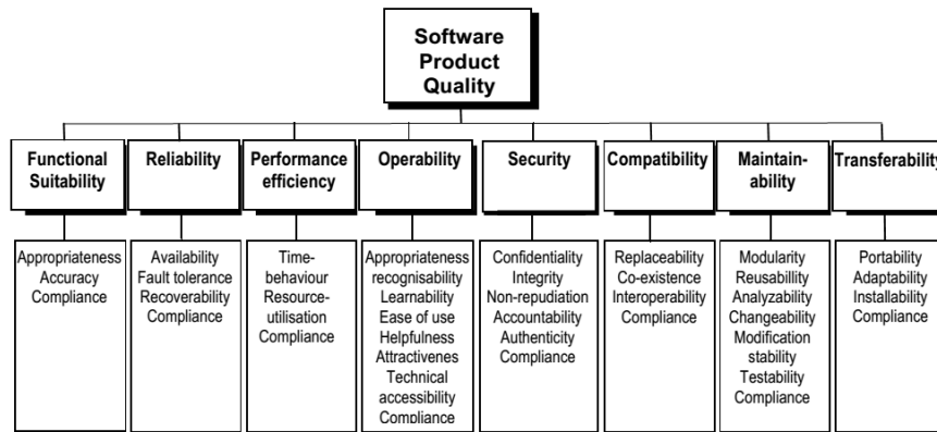
Figure 1. Software Product Quality as defined in ISO 25010
