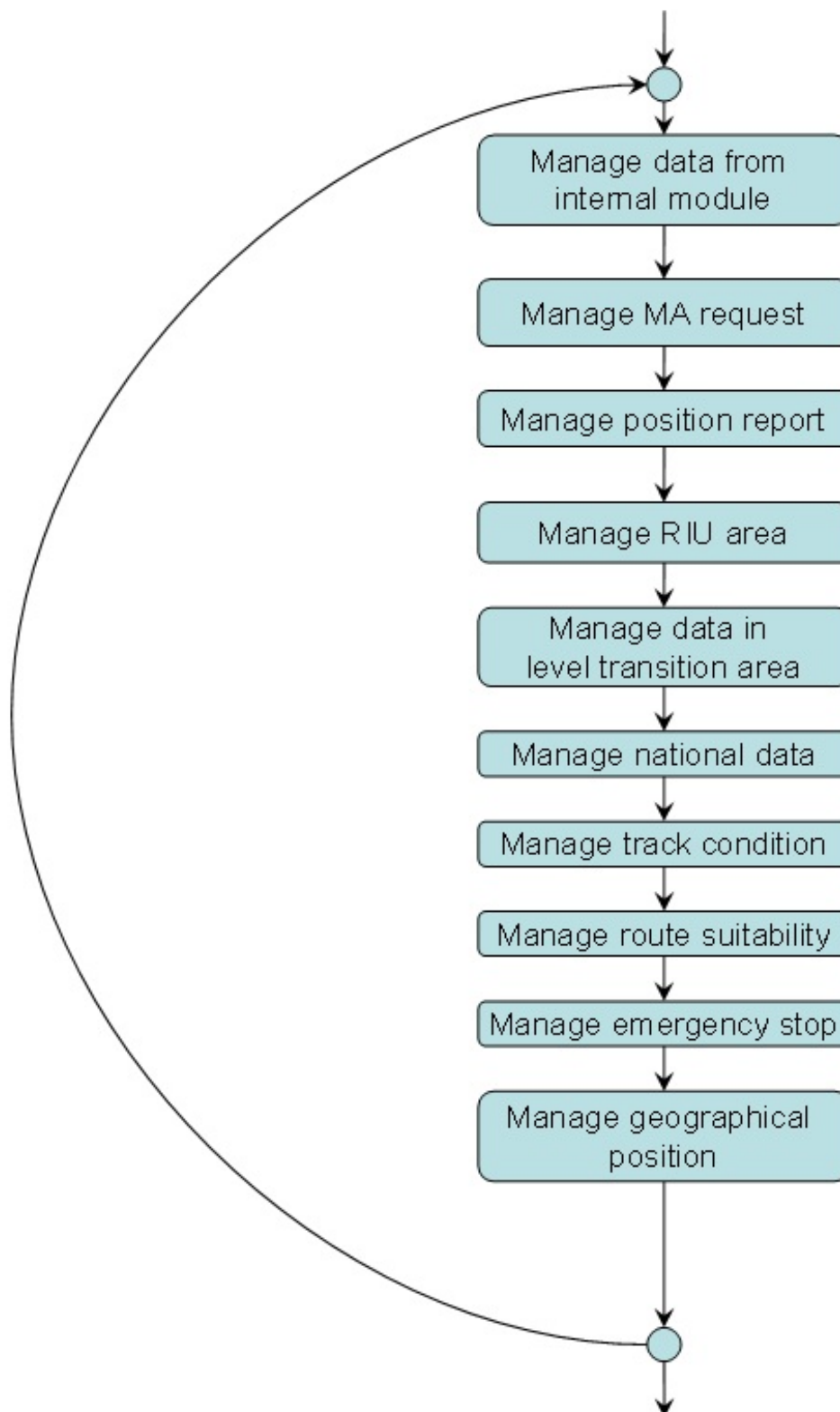
Figure 10. Data manager, sequence diagram
