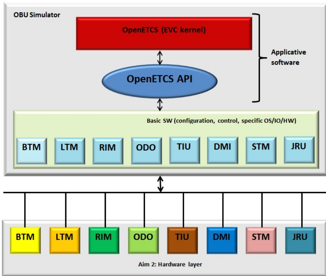
Figure 7. Use of API in the Demonstrator
