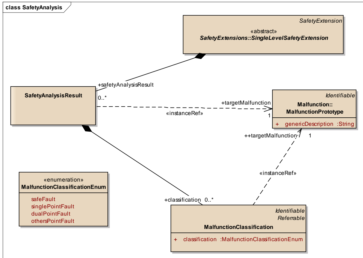
Figure 65: SafetyAnalysis - (Class diagram)
