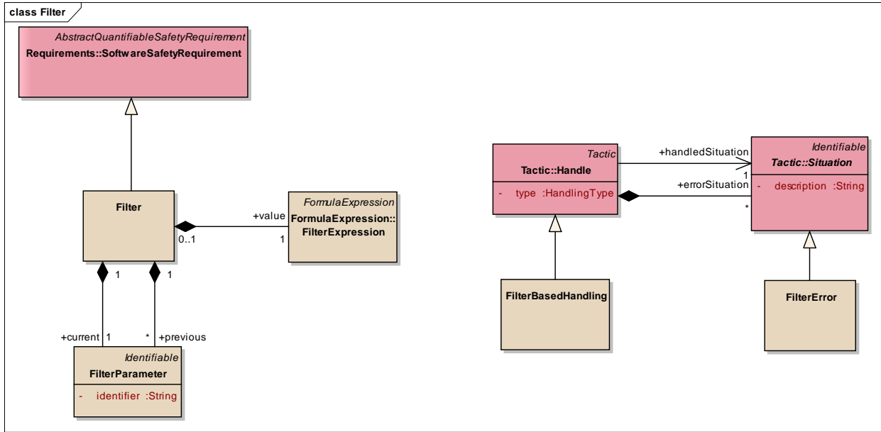
Figure 57: Filter - (Class diagram)
