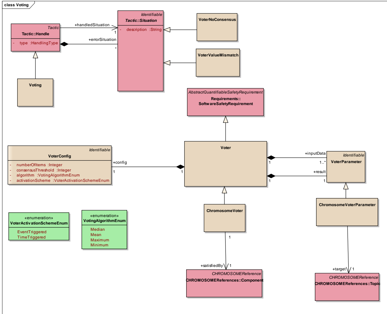
Figure 63: Voting - (Class diagram)
