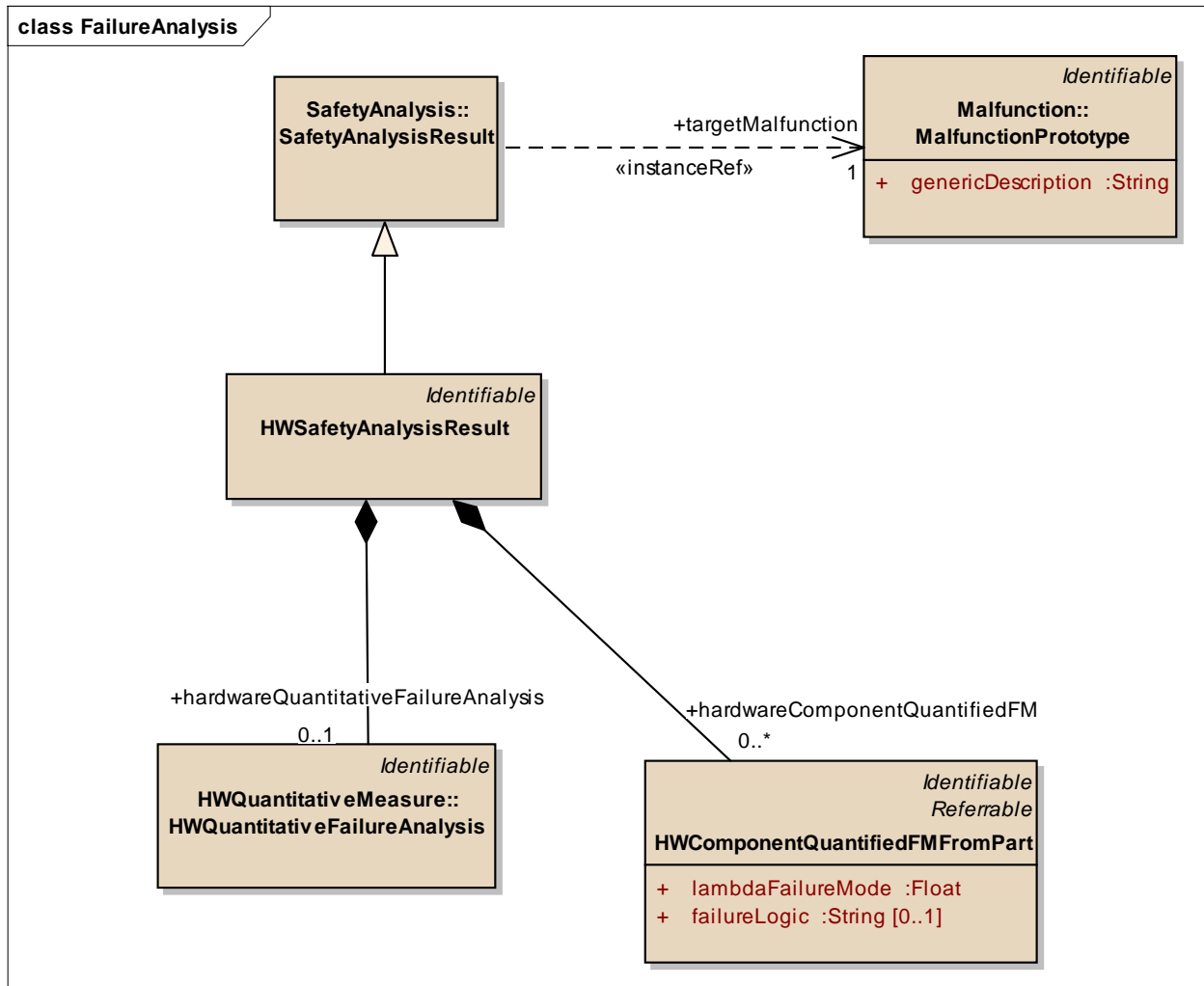
Figure 33: FailureAnalysis - (Class diagram)
