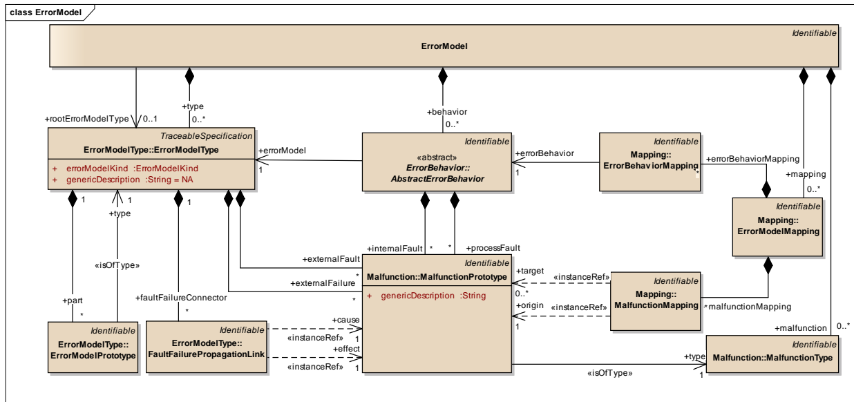
Figure 16: ErrorModel - (Class diagram)
