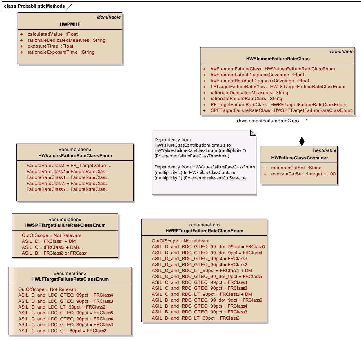
Figure 41: ProbabilisticMethods - (Class diagram)
