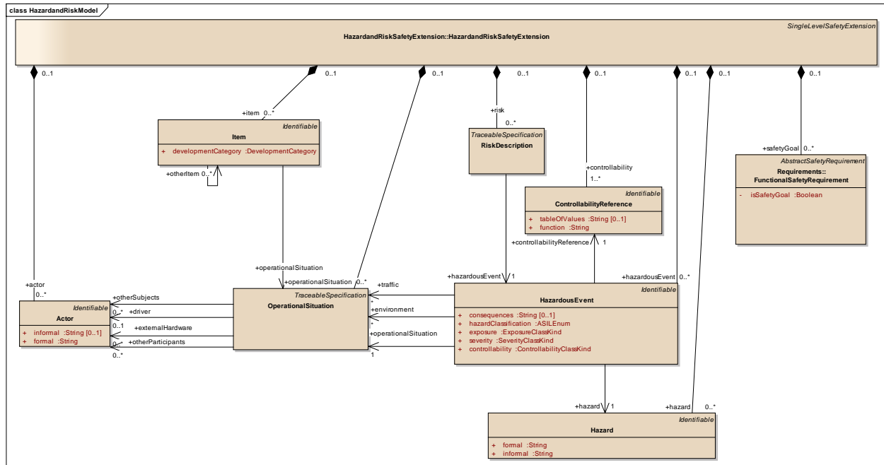
Figure 43: HazardandRiskModel - (Class diagram)
