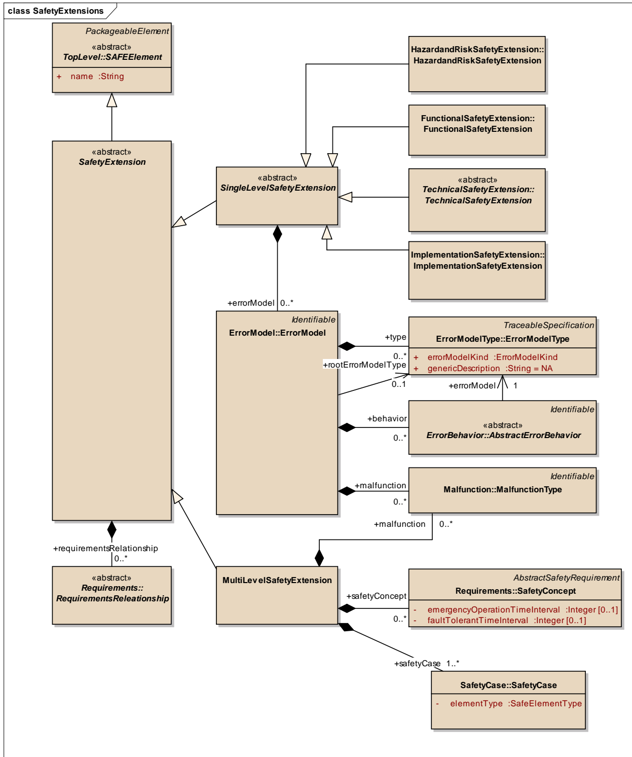
Figure 9: SafetyExtensions - (Class diagram)
