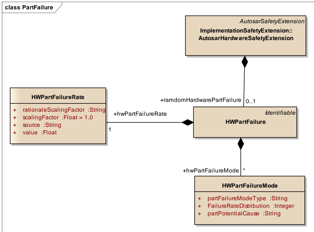
Figure 36: PartFailure - (Class diagram)
