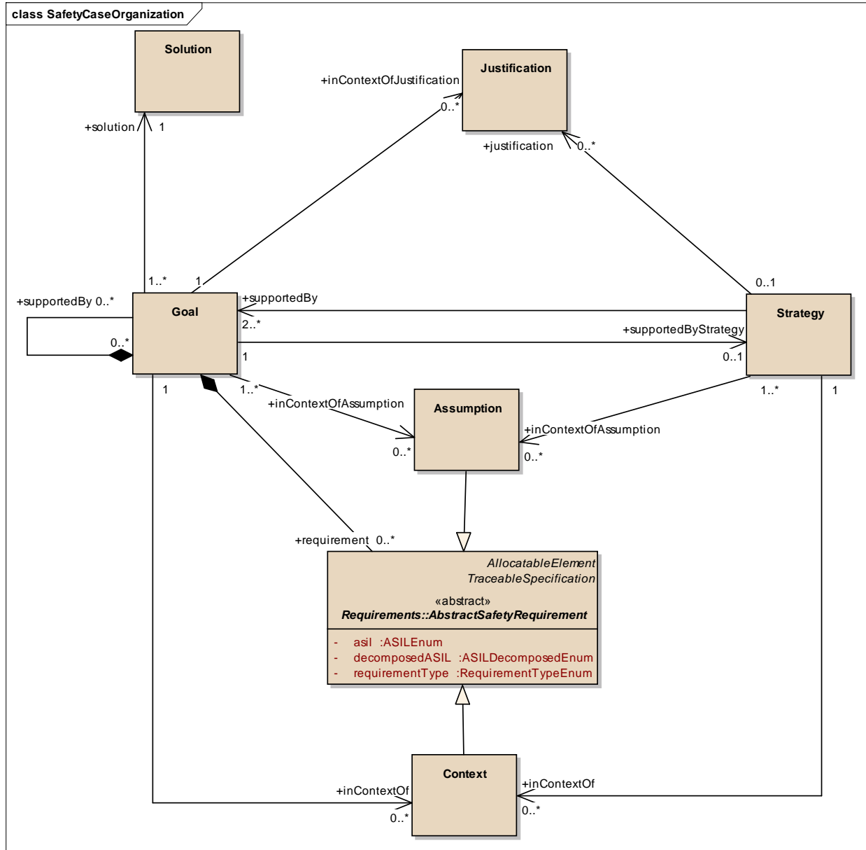
Figure 48: SafetyCaseOrganization - (Class diagram)
