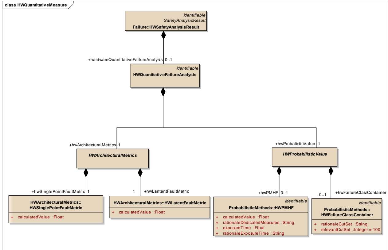
Figure 40: HWQuantitativeMeasure - (Class diagram)
