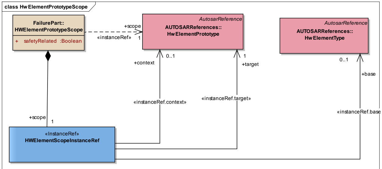
Figure 39: HwElementPrototypeScope - (Class diagram)
