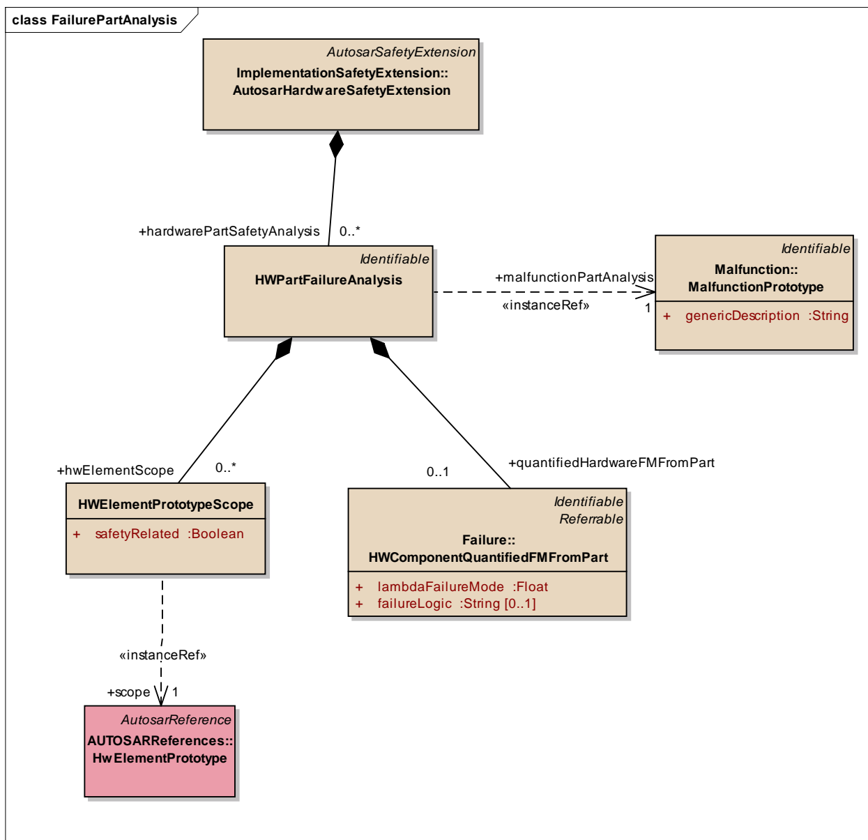
Figure 35: FailurePartAnalysis - (Class diagram)
