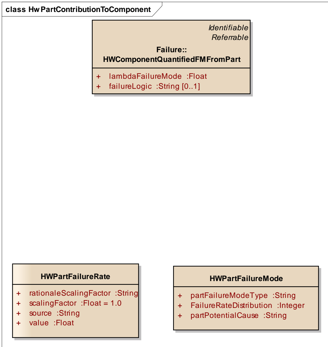
Figure 37: HwPartContributionToComponent - (Class diagram)
